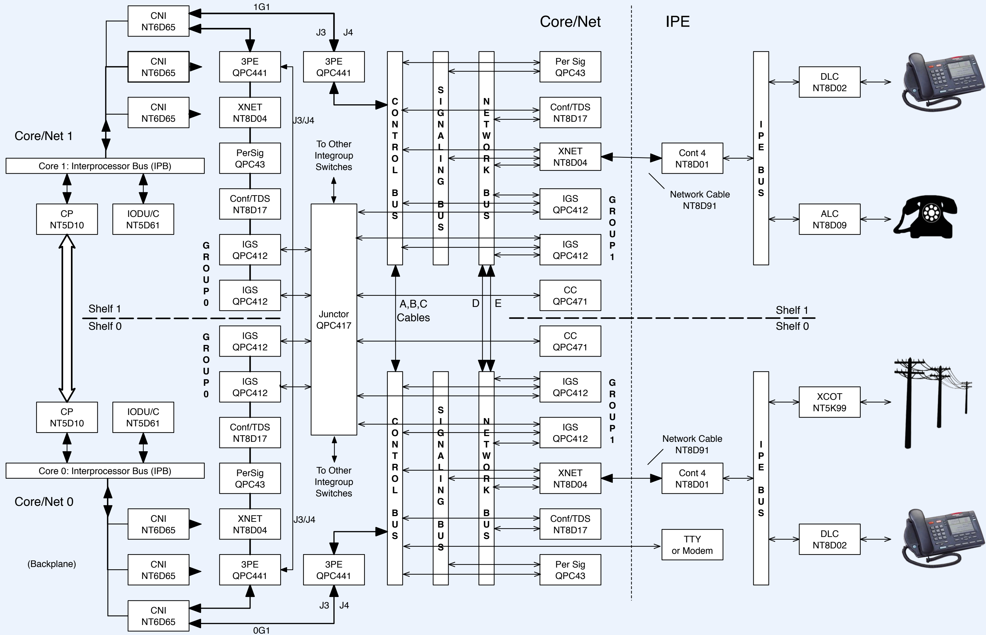
Option 81C Block Diagram
