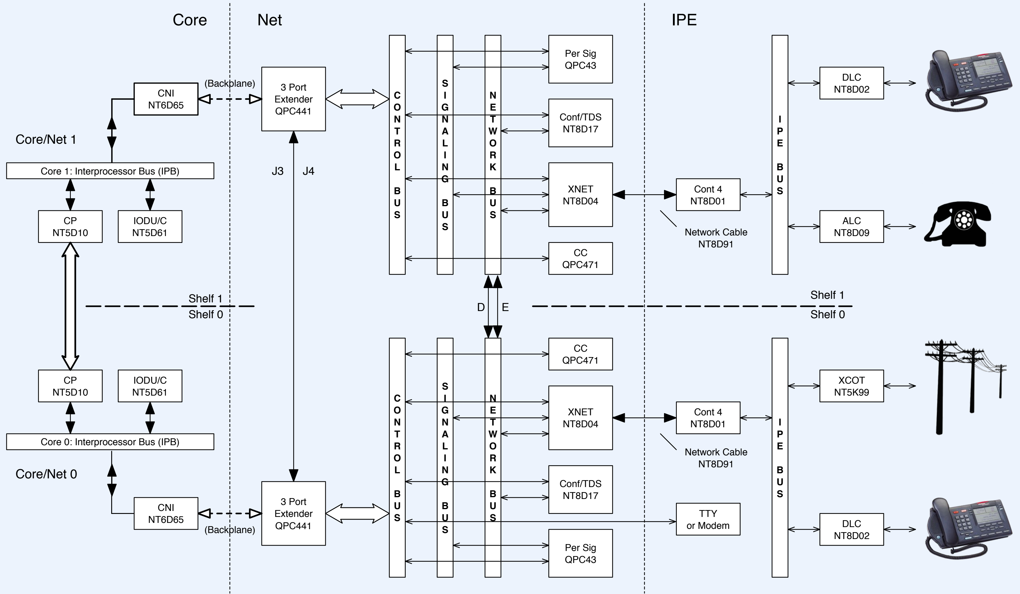
Option 61C Block Diagram
